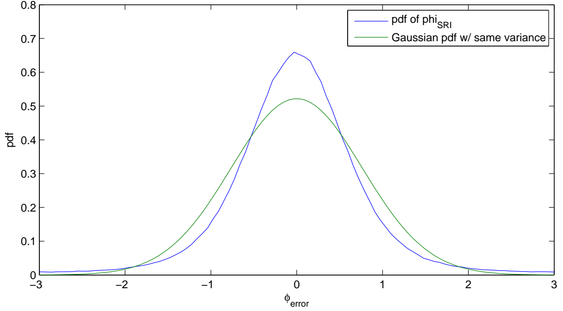
Figure 45: Empirical pdf of \phi_{SRI} with high noise
