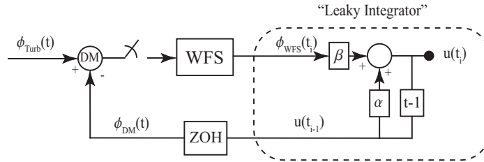
Figure 32: Block diagram of a leaky integrator
