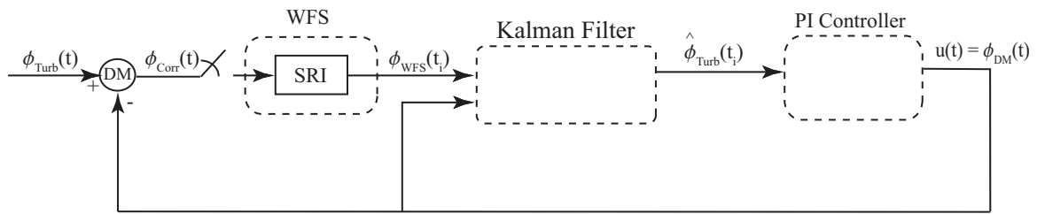
Figure 34: Optimal control structure block diagram
