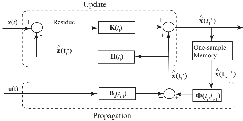
Figure 16: Kalman filter illustration [30]
