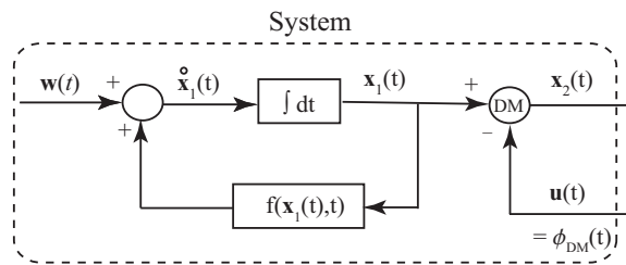
Figure 33: Stochastic model of turbulence with DM
