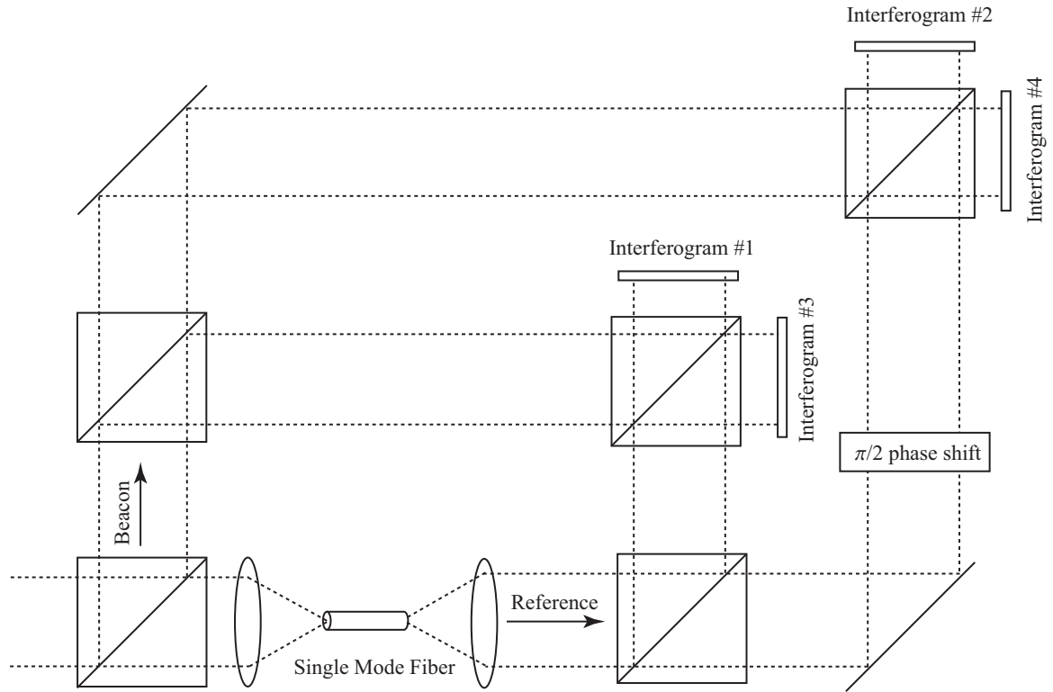
Figure 10: Conceptual Spatially Designed SRI [37]
