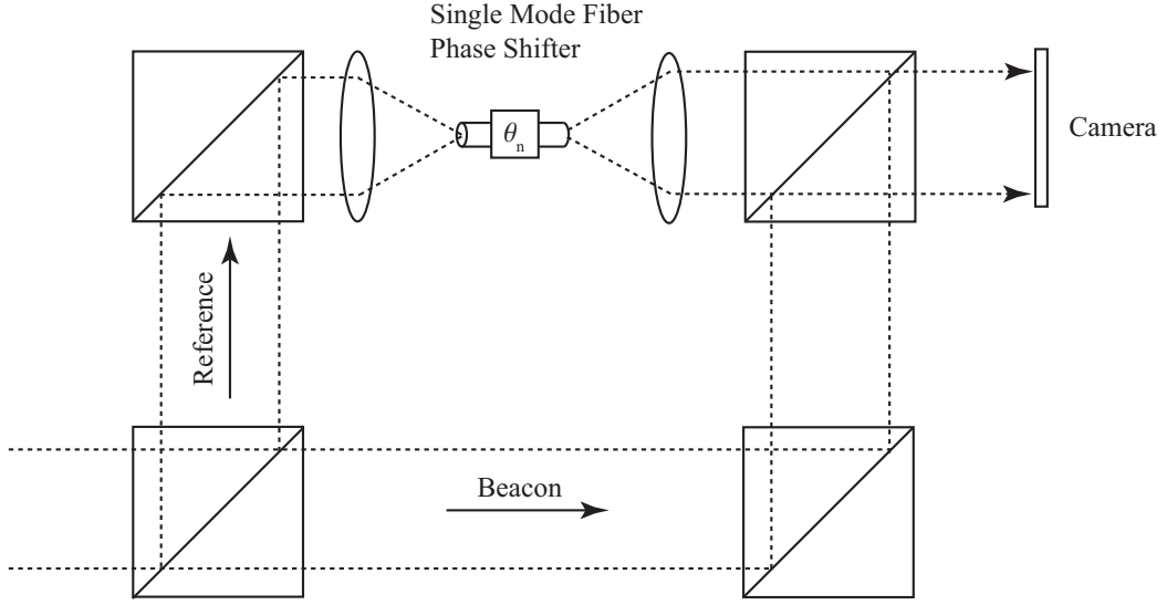
Figure 9: Conceptual diagram of a temporally phase-shifted SRI [35]
