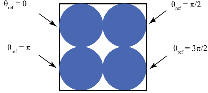
Figure 12: Spatial SRI [34]
