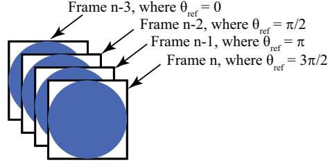
Figure 11: Frame sequence for a temporal SRI [38]. The black outline indicates the extent of the camera. The blue circle is the area of the pupil interferogram.
